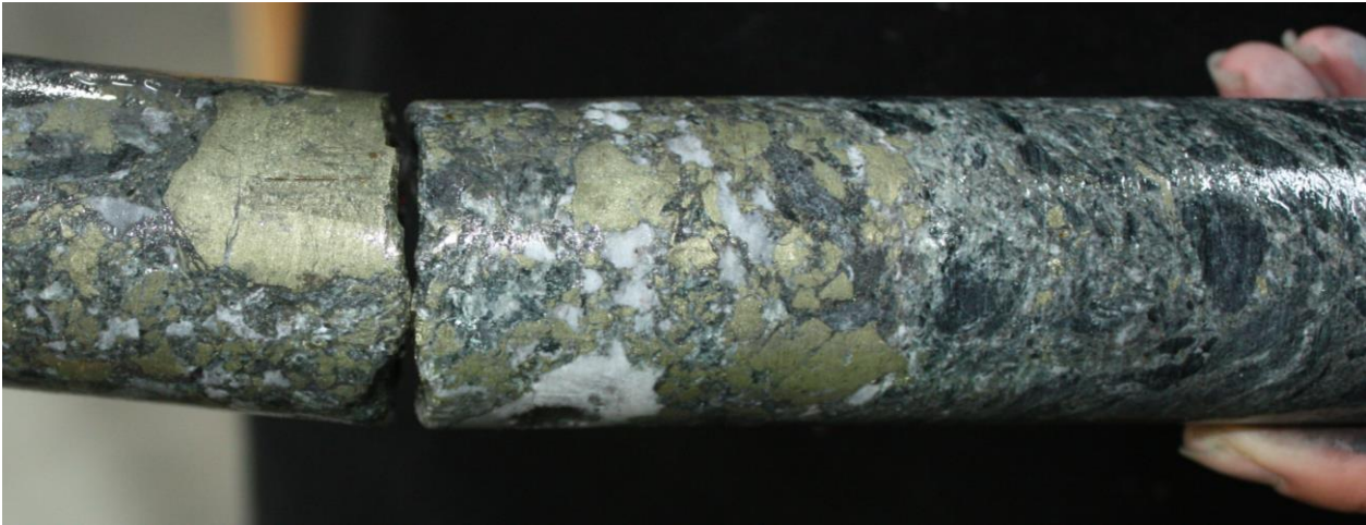
Figure 4: VDD 186 drill core at 536.2m showing breccia texture with significant chalcopyrite. VDD 186 was drilled from a collar position of 1,680,986mE and 7,537,063mN, at an RL of 536m, at a dip of -55 degrees and an azimuth of 310 degrees, and end of hole of 563.2m
