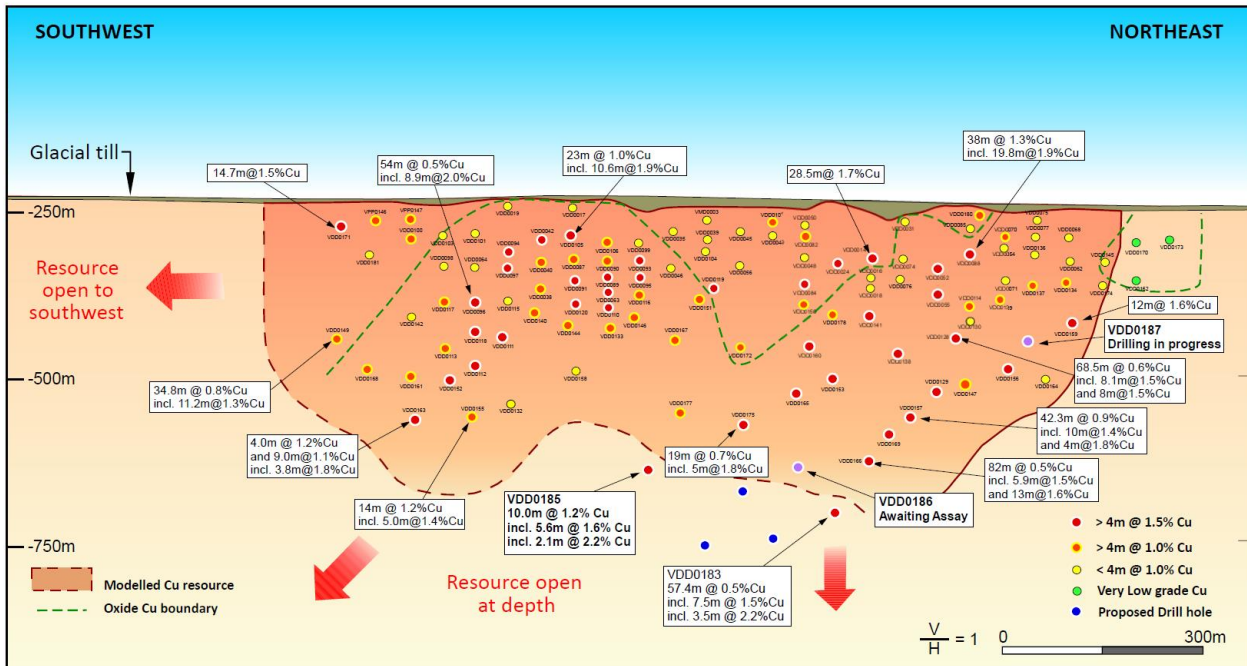
Figure 2 – Location on schematic long section of VDD 183, 185, 186 and 187 at the Viscaria Copper Project, D Zone.
