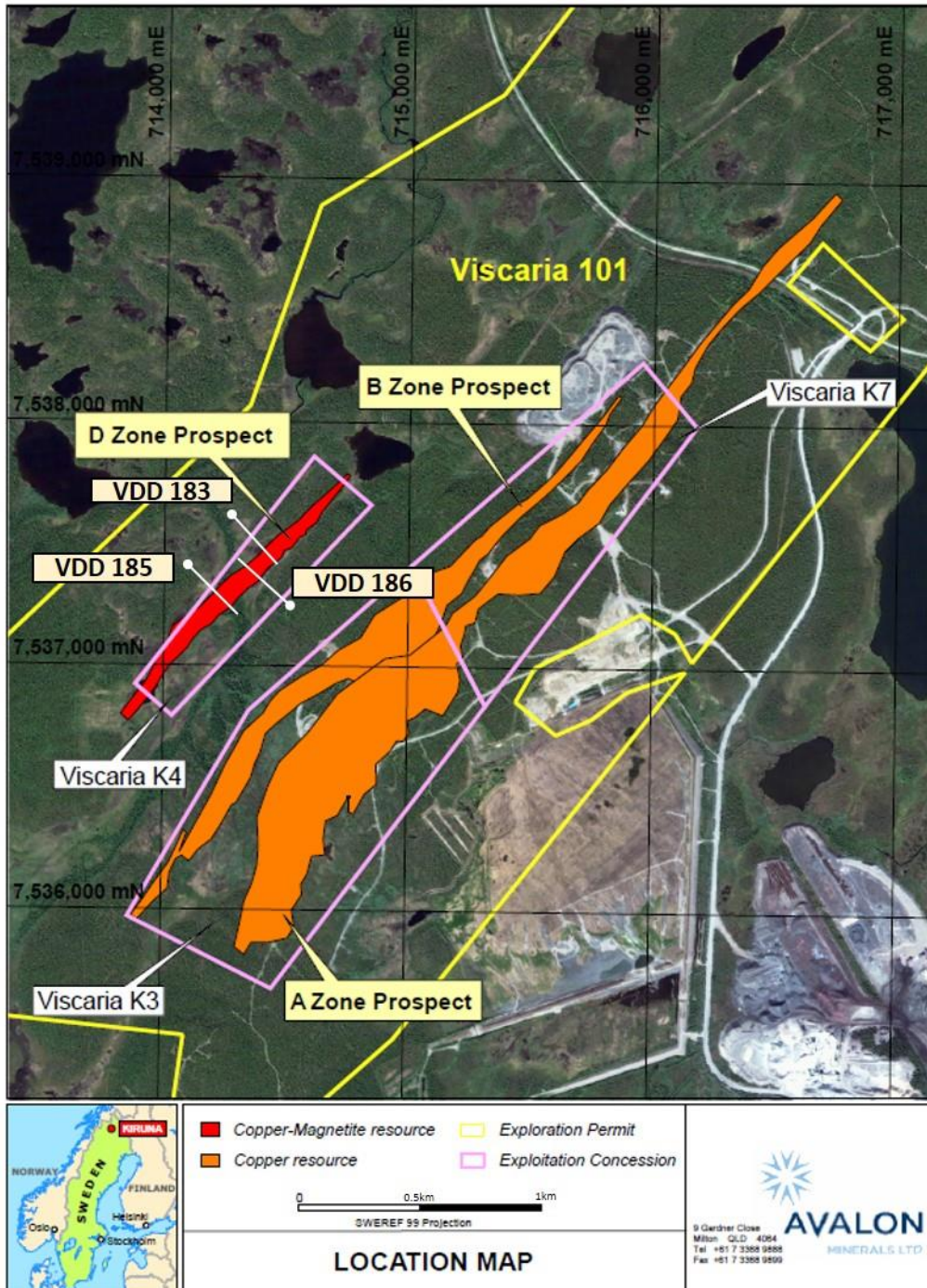
Figure 1 – Location of VDD 183, 185, and VDD 186 at the Viscaria Copper Project, D Zone
