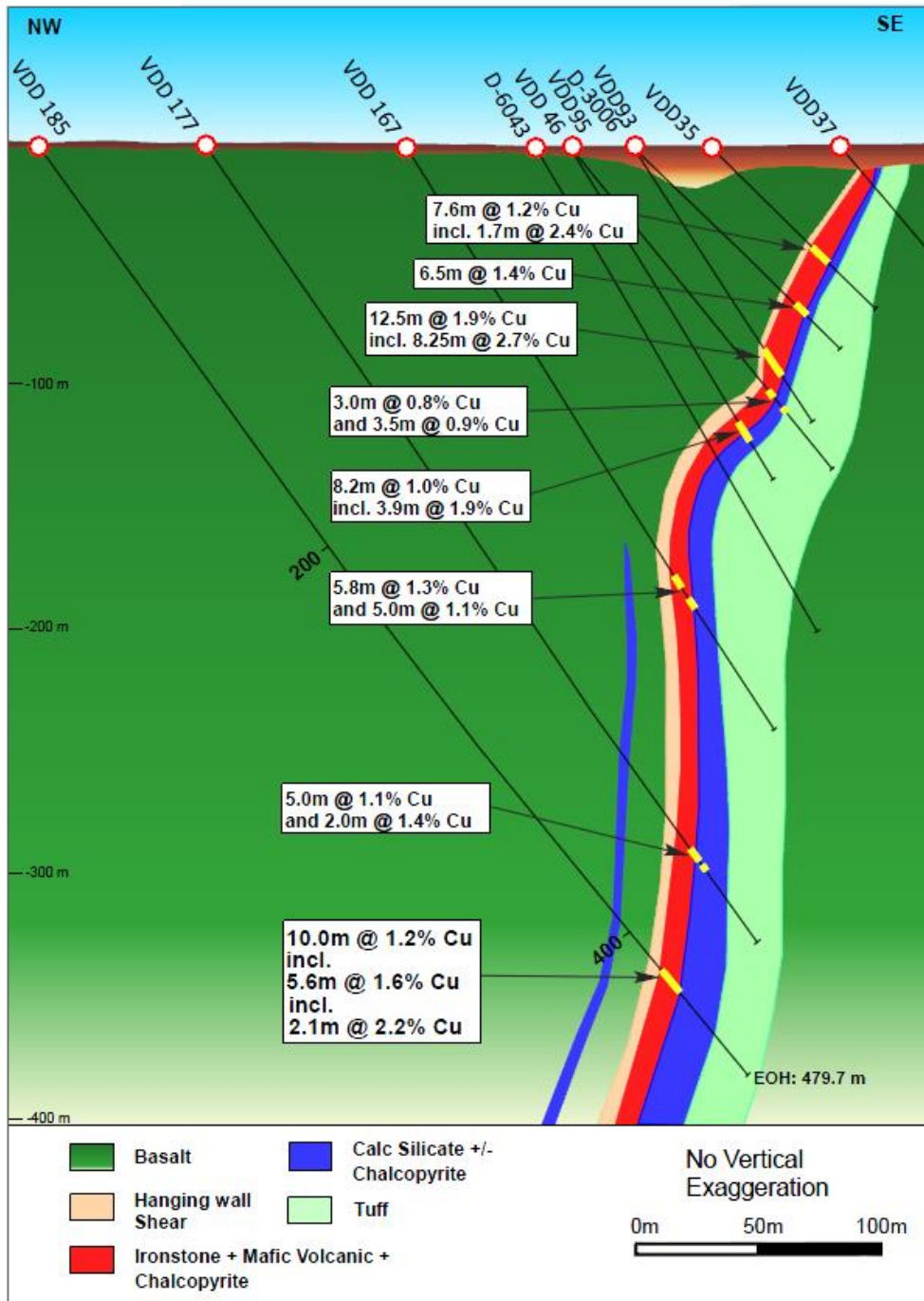
Figure 3: Drill hole cross section containing VDD 185 and previously drilled diamond holes. VDD 185 is collared at 1680120mE and 7537014mN, at an RL of 521m.
