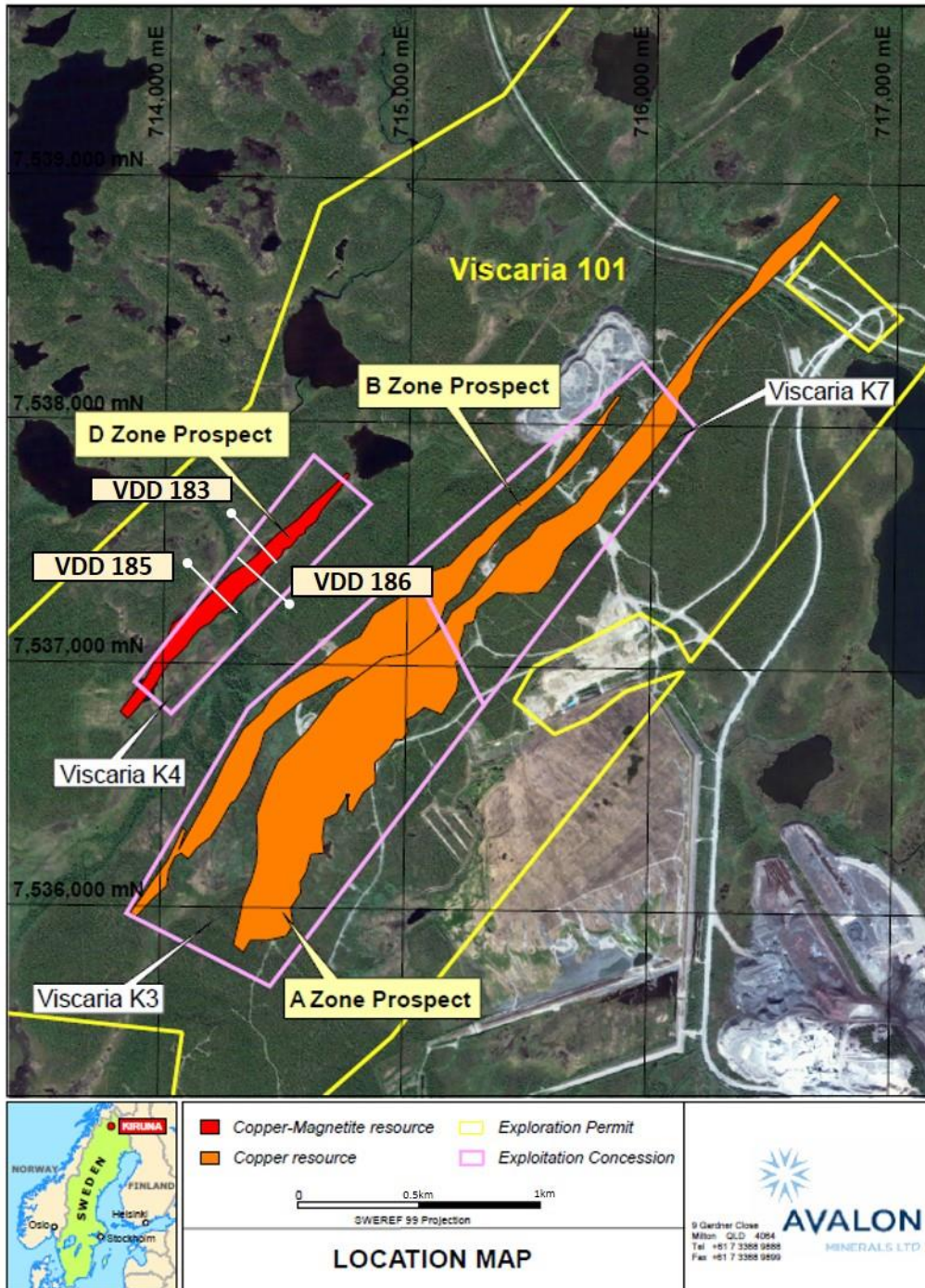
Figure 1: Location of VDD 186 at the Viscaria Copper Project, D Zone
